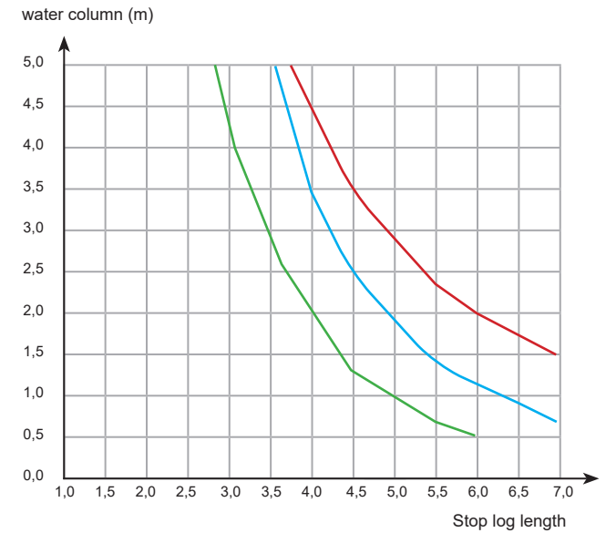
Stop log profile 225 x 150 mm
