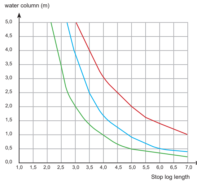
Stop log profile 150 x 90 mm
