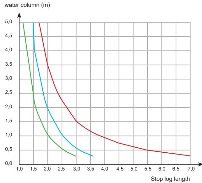
Stop log profile 300 x 50 mm
