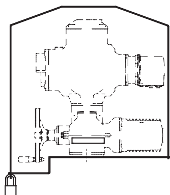
Cover for e-actuator with control unit
