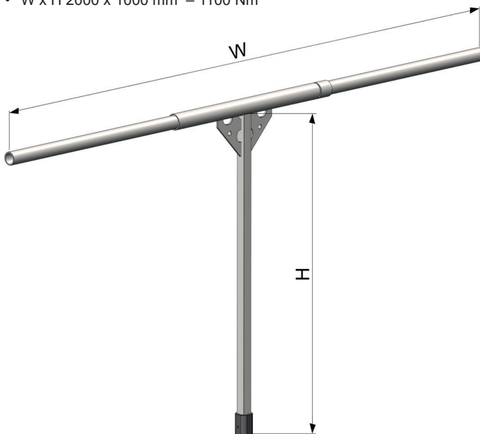
View Symmetrical operation by two persons
