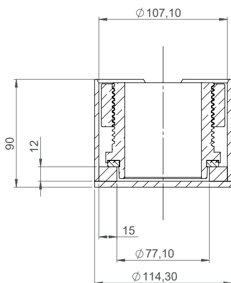
Standpipe hygiene lock cap® with mounted Street cap cleaner
